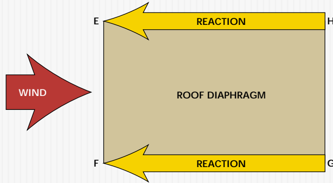
FIGURE 3 Roof diaphragm provides resistance to lateral loads
