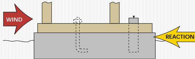
FIGURE 5a Shear wall anchor bolts – transfer shear forces into foundation
