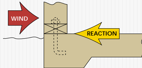
FIGURE 2a Perimeter anchor bolts – transfer forces into foundation
