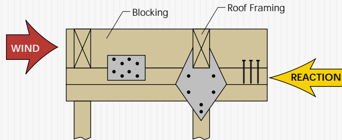
FIGURE 3a Roof to wall connections – fasteners must be able to transfer forces between roof and walls
