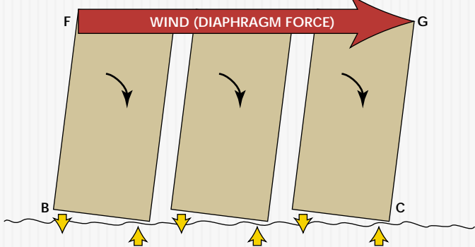
FIGURE 6 Overturning forces
