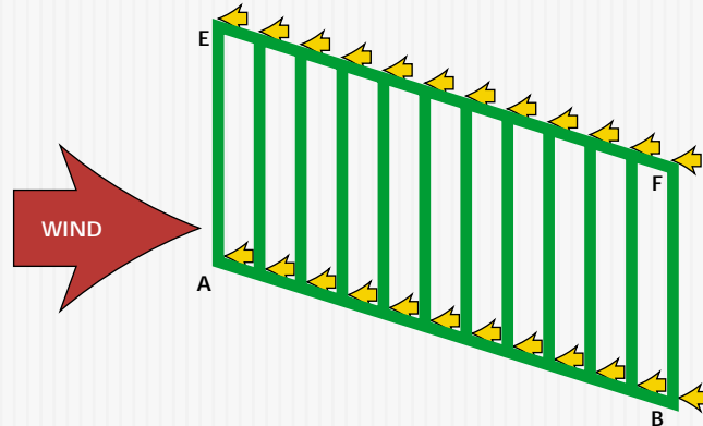
FIGURE 2 Lateral load acting on an end wall and transfer of resulting forces
