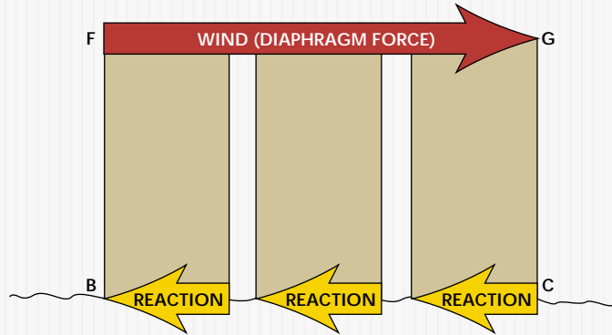
FIGURE 5 Reaction of segments in shear wall with openings
