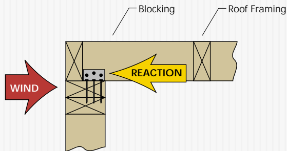
FIGURE 2b Rafter connection detail – transfers forces into diaphragm
