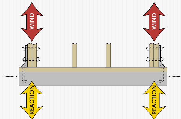
FIGURE 6a Holddown anchors – transfer overturning forces into foundation
