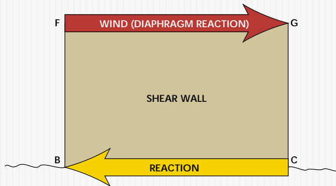
FIGURE 4 Shear wall reaction to lateral loads
